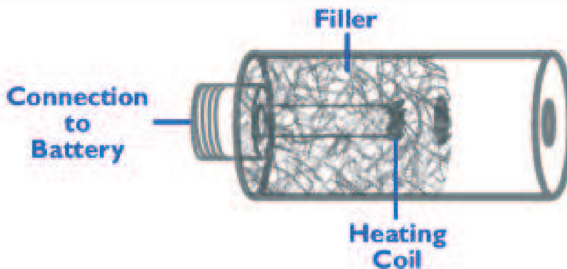
Cartomizer Components
